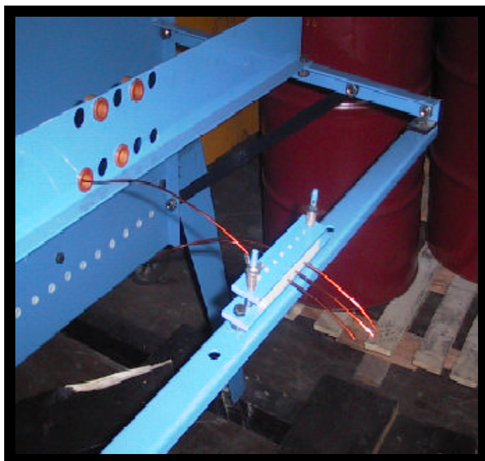
Illustrates Model 44-TD mounted to Model 41 Wire Rack
